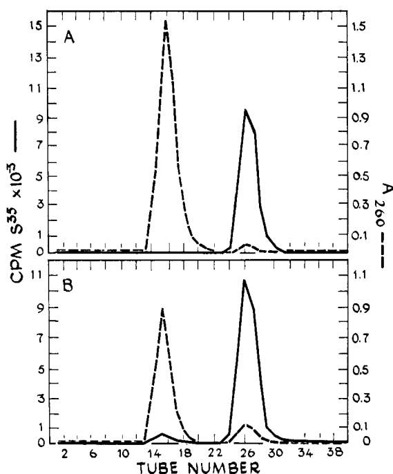
FIGURE 2: Separation of polyuridylic acid from [ 35 S]-cysteine on Bio-Gel P-2. Columns (0.8 × 35 cm) packed with 200–400 mesh gel (exclusion limit mol wt 1600) were eluted with 0.15 M NaCl at the rate of 0.5 ml every 2 min. (a) Before ultraviolet irradiation of the [ 35 S]-cysteine-poly rU mixture. (b) After 60-min ultraviolet irradiation.
