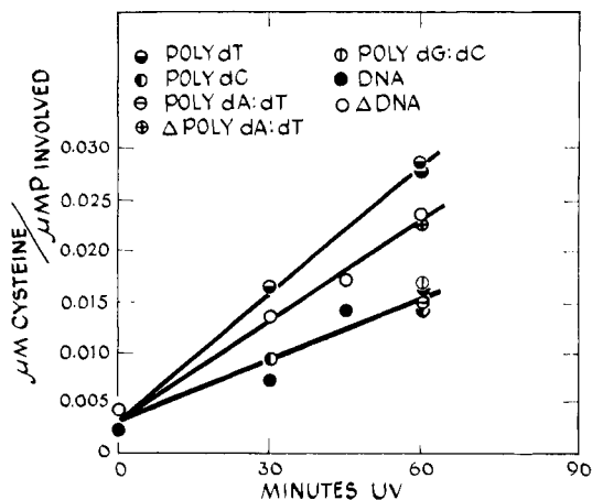
FIGURE 4: Photochemical addition of [ ^{35}\text{S} ]cysteine to DNA, poly dT, poly dC, poly dC:dG, and poly dA:dT. \Delta = heated for 15 min at 100^\circ and quick cooled before irradiation.
