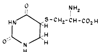
FIGURE 1: 5-S-cysteine-6-hydrouracil.
